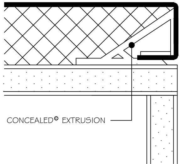
EDGE @ OUTSIDE CORNER
