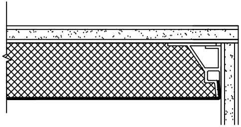
Ⓐ 2" NOVASPAN 16 @ INSIDE CORNER
