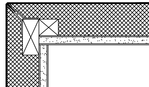
Ⓖ 2" NOVASPAN 16 @ OUTSIDE CORNER
