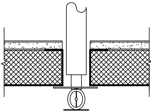
Ⓒ 2" NOVASPAN 16 @ INSIDE CORNER
