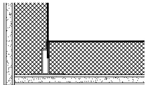
Ⓒ 2" NOVASPAN 16 @ INSIDE CORNER
