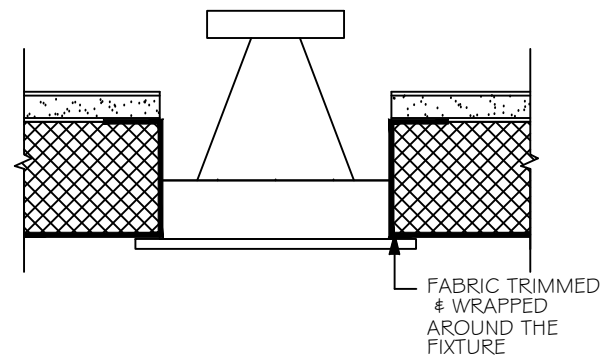
Ⓖ 2" NOVASPAN 16 @ LIGHT FIXTURE
