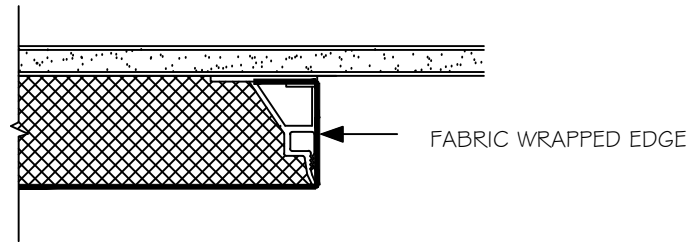
Ⓕ 2" NOVASPAN 16 @ EXPOSED EDGE (REF. N/A)
