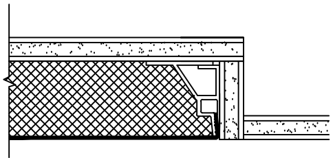
Ⓑ 2" NOVASPAN 16 @ FLUSH MOUNT
