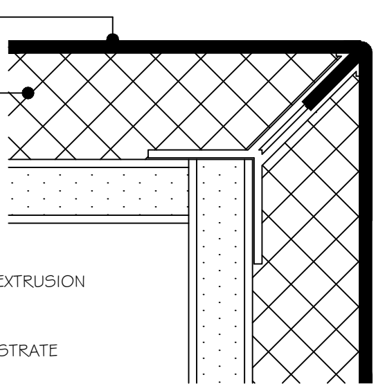
EDGE @ OUTSIDE CORNER
