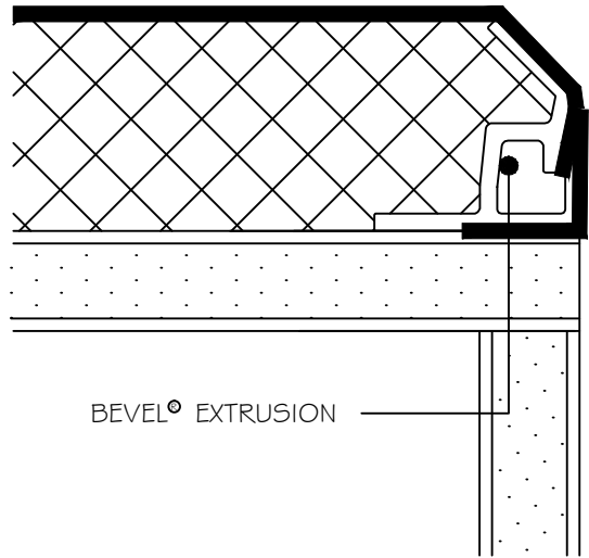
EDGE @ OUTSIDE CORNER
