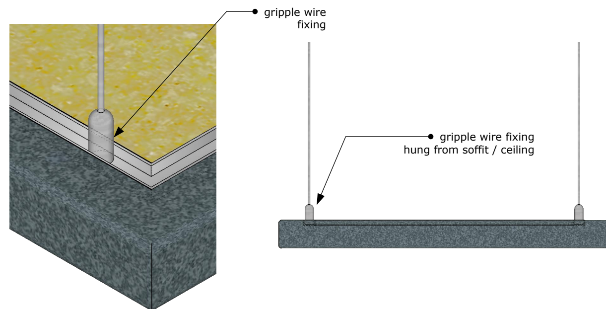
Corner Detail
