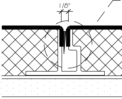
MIDSEAM
