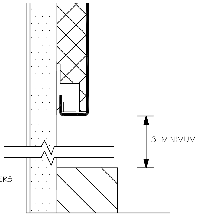
CONCEALED @ WOOD BASE
