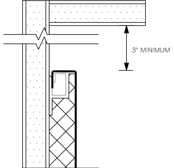
CONCEALED @ CEILING
