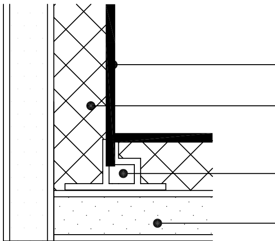
INSIDE CORNER
