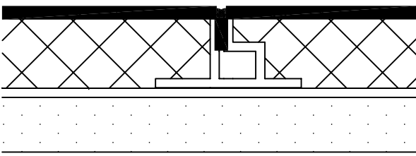
MIDSEAM
