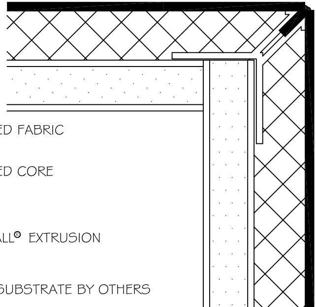
OUTSIDE CORNER
