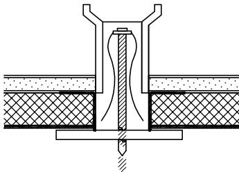
(E) 1" NOVASPAN 10 @ INSIDE CORNER
