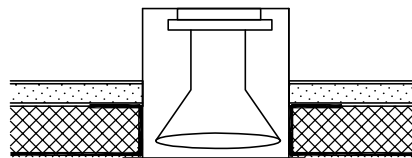
(F) 1" NOVASPAN 10 @ OUTSIDE CORNER
