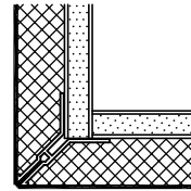
(F) 1" NOVASPAN 10 @ OUTSIDE CORNER
