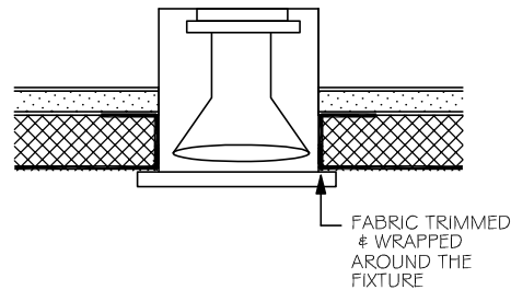
(H) 1" NOVASPAN 16 @ TYPICAL LIGHT
