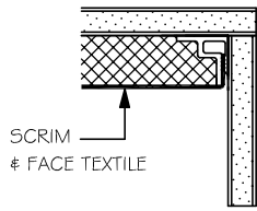
(A) 1" NOVASPAN 16 @ WALL
