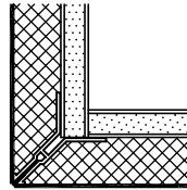
(F) 1" NOVASPAN 16 @ OUTSIDE CORNER
