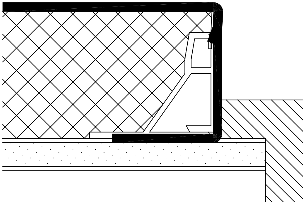
2" WELTLESS @ DOOR FRAME
