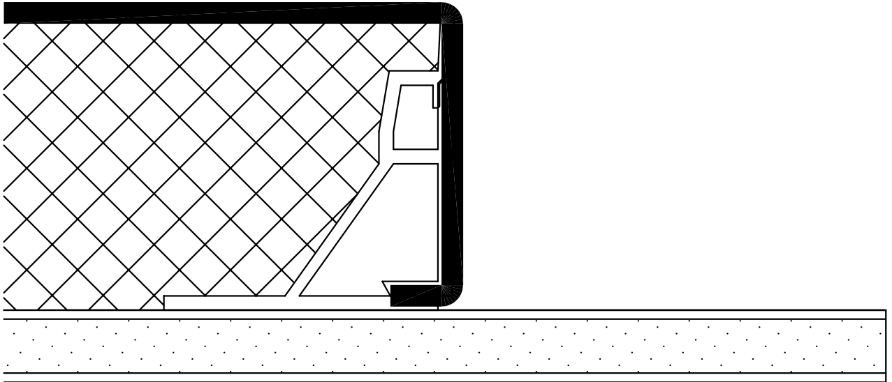
2" SIDELOAD EXPOSED
